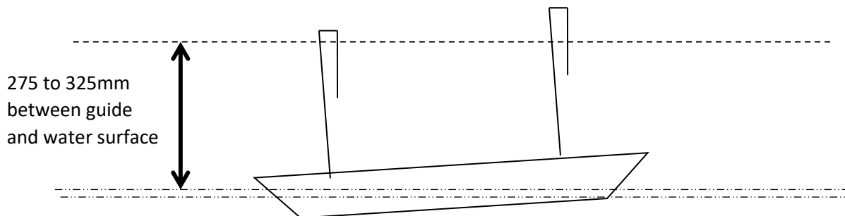
Figure 2: guide wire height and guide rod position
